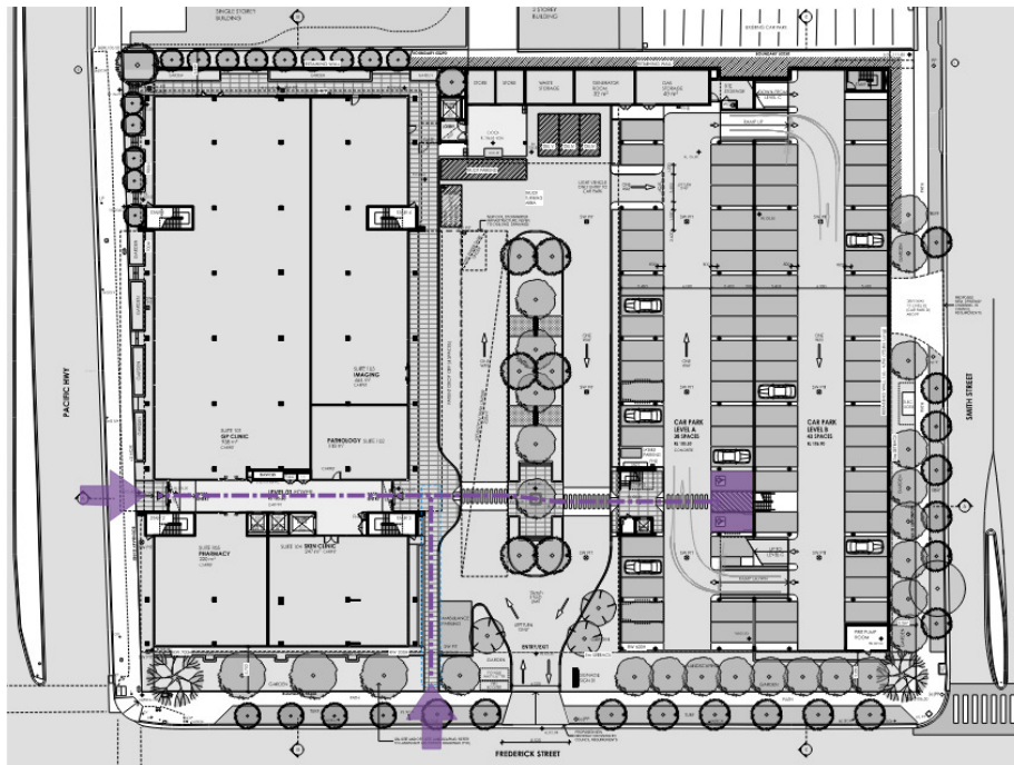
Figure 2 | Level 1 Plan
